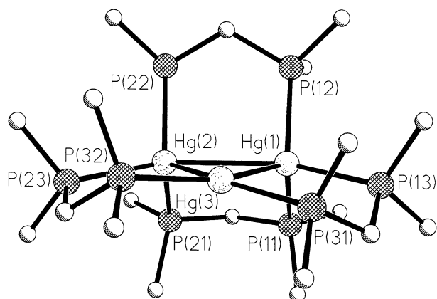
Fig. 1 View of [\text{triangulo-Hg}_3(\mu\text{-dmpm})_4]^{4+} \mathbf{2}
