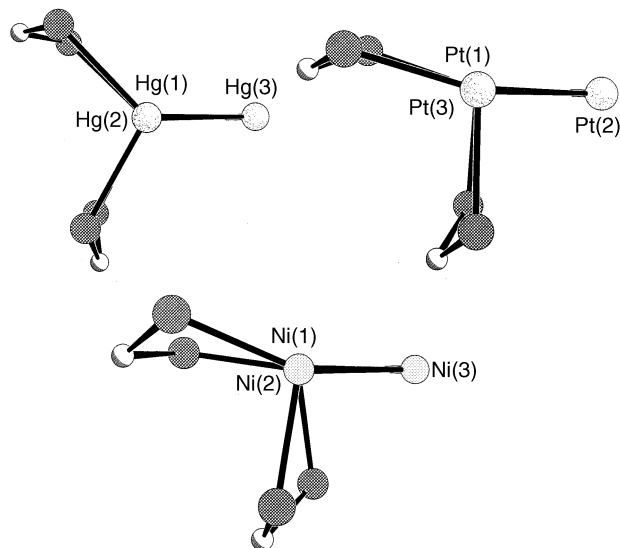
Fig. 2 View along the vector of the doubly bridged Hg atoms of [\text{triangulo-Hg}_3(\mu\text{-dmpm})_4]^{4+} \mathbf{2} and analogous projections of [\text{triangulo-}[\text{Pt}_3(\mu\text{-CO})(\mu\text{-dmpm})_4]^{2+} \mathbf{3} and [\text{triangulo-Ni}_3(\mu_3\text{-CO})(\mu\text{-dmpm})_4]^{2+} \mathbf{4} showing the different co-ordination geometries of the doubly bridging dmpm ligands
